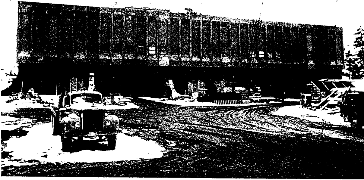
Figure 2. West ventilation building under construction.
