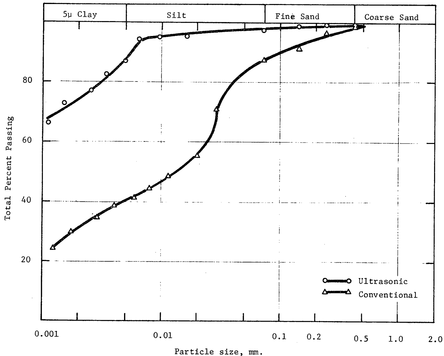
Figure 7. Grain-size distribution of shale no. 19.
