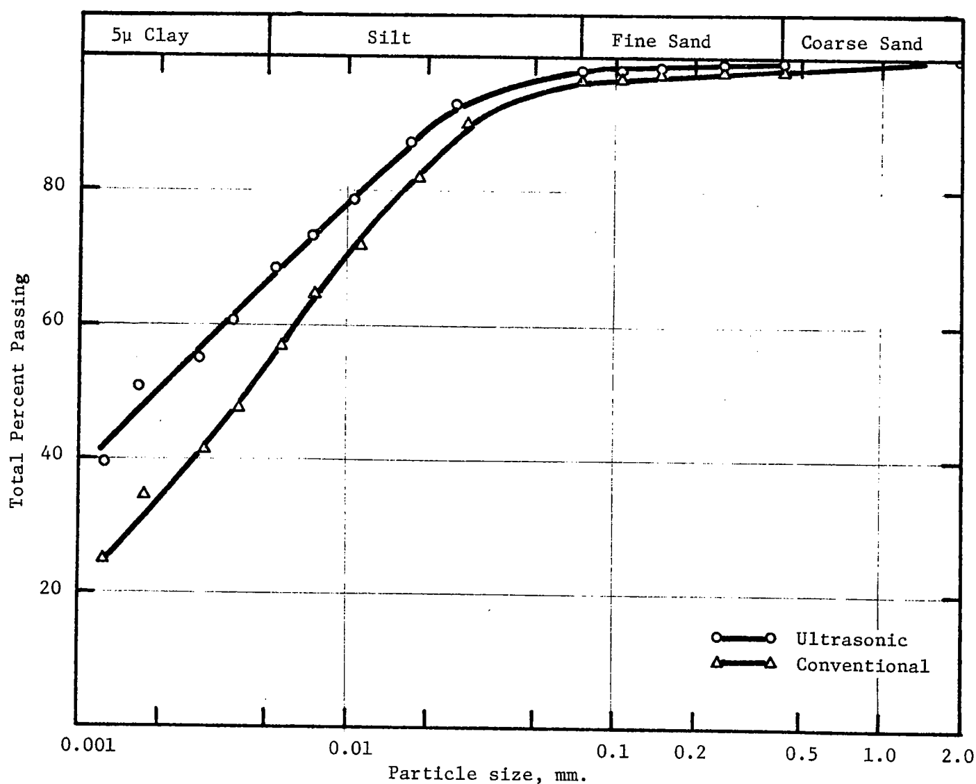
Figure 8. Grain-size distribution of shale no. 23.
