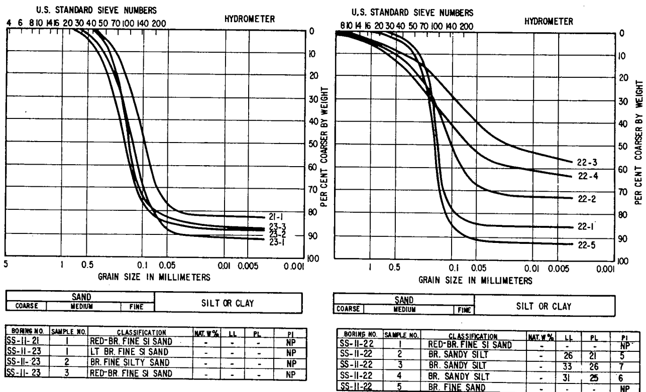
Figure 11. Mechanical analysis and Atterberg limits.
