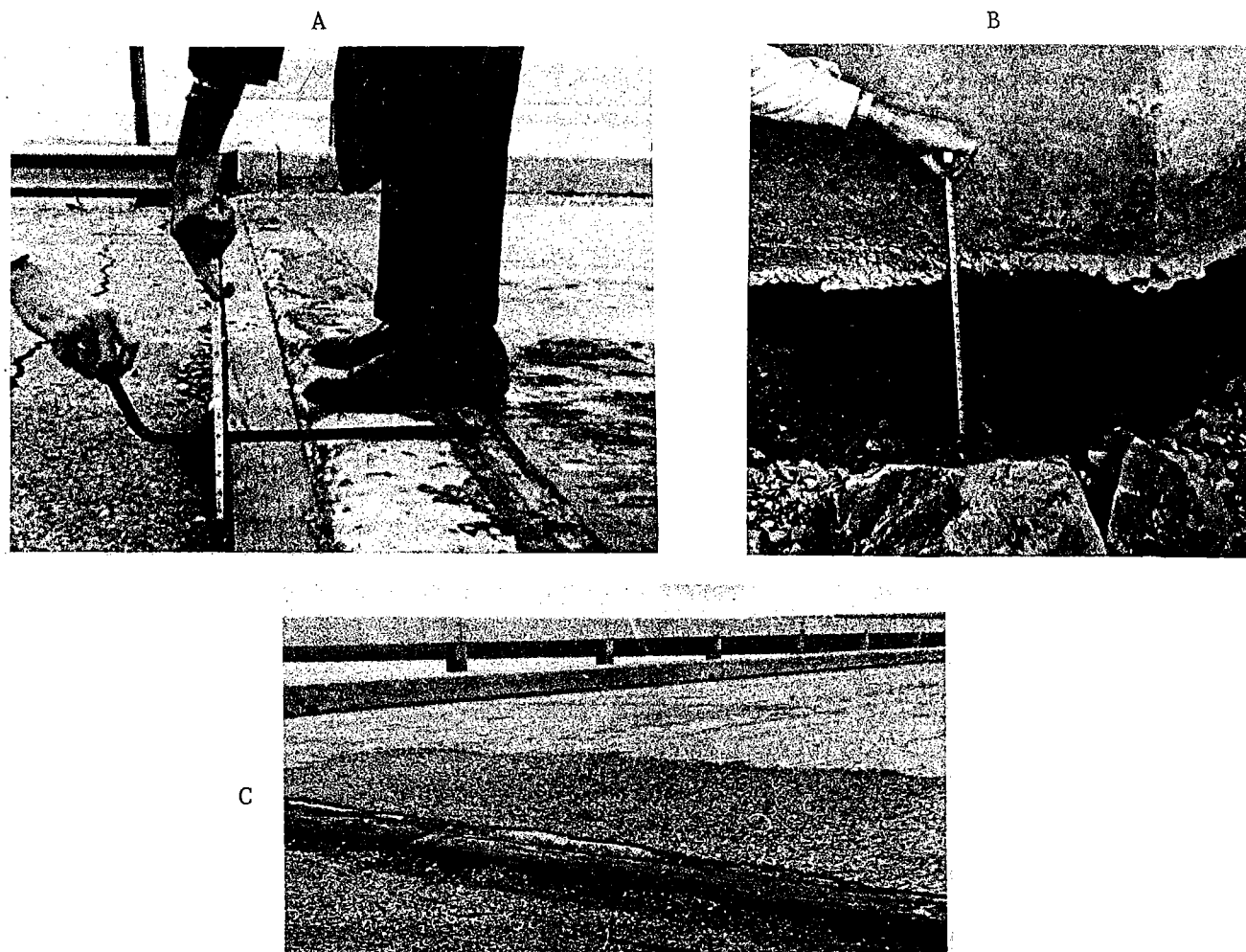
Figure 6. Evidence of settlement. A. Settlement of approach fill at abutment no. 1, about 5 inches. B. Settlement of approach fill at abutment no. 2, about 4 inches. C. Settlement at base of abutment seat, about 18 inches in April 1968. Note exposed piling.
