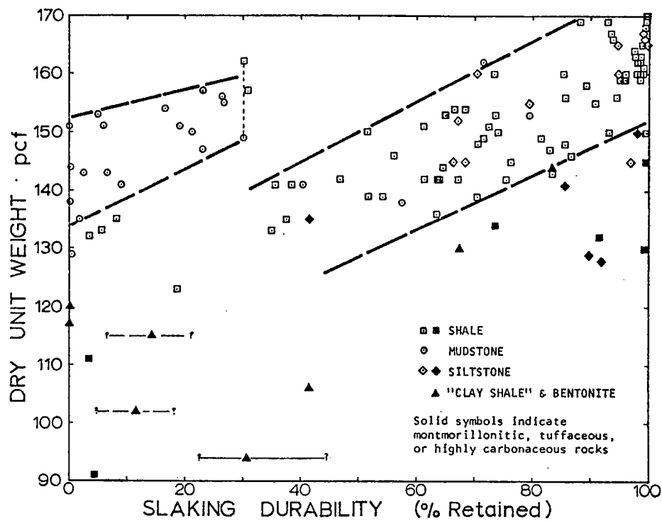
Figure 1. Dry unit weight vs. slaking durability.
