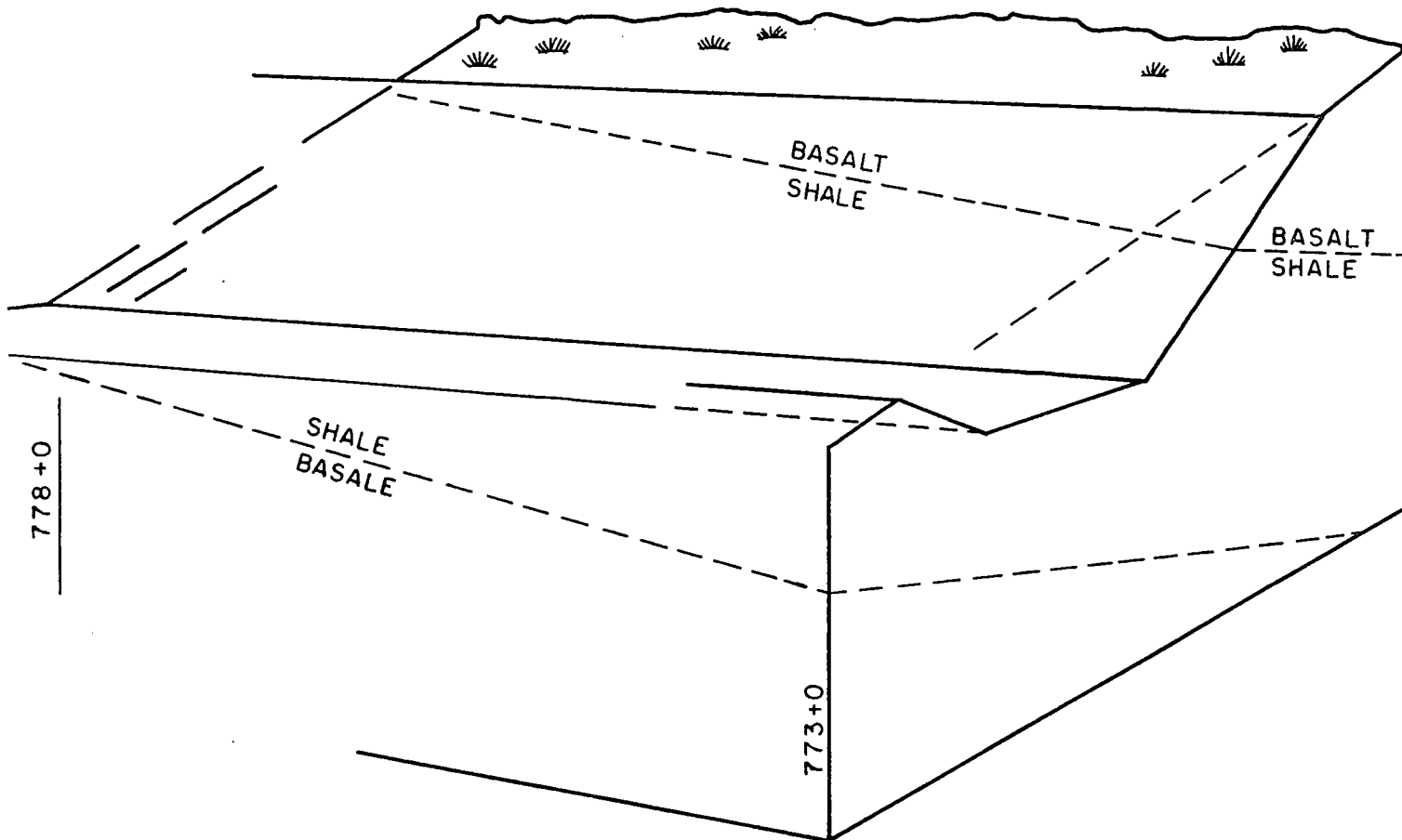
Figure 1. Perspective of Test Cut 775.
