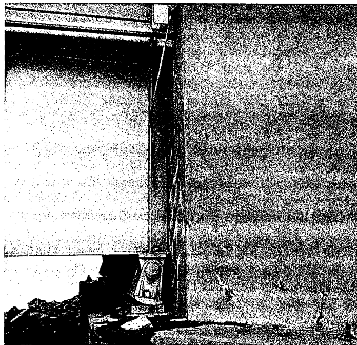
Figure 3. Plate girder restraining horizontal movement of abutment. Note position of rockers.
