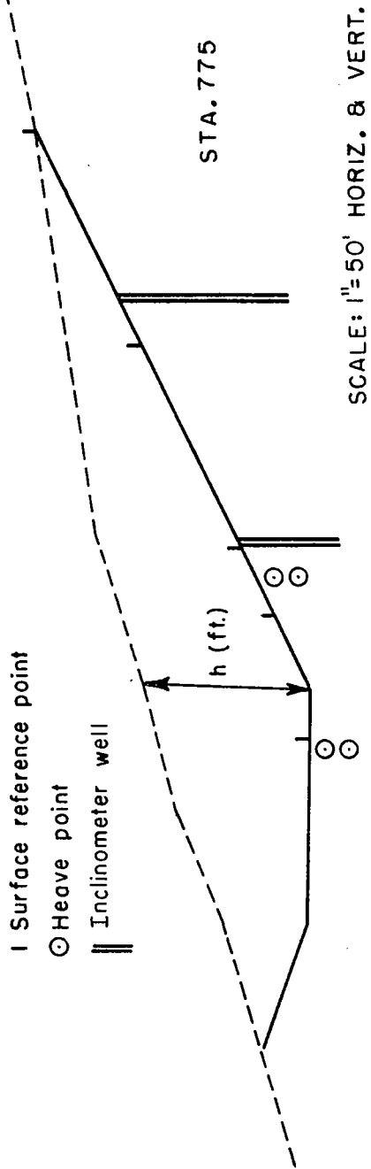
Figure 2. Typical cross section of test cut.
