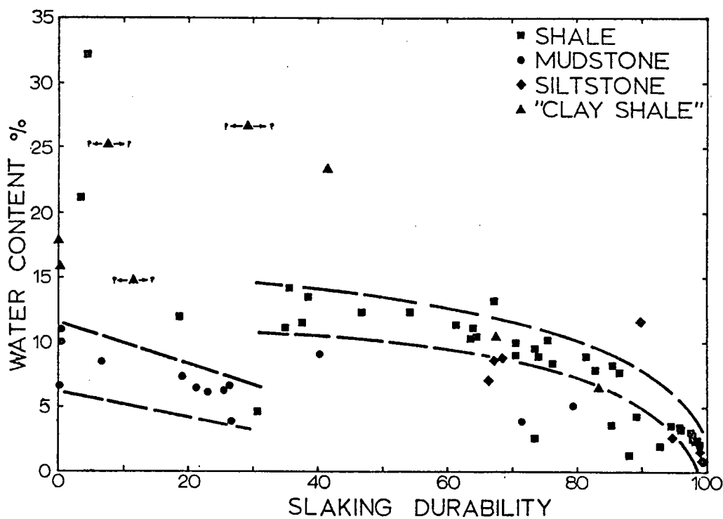
Figure 2. Water content vs. slaking durability.
